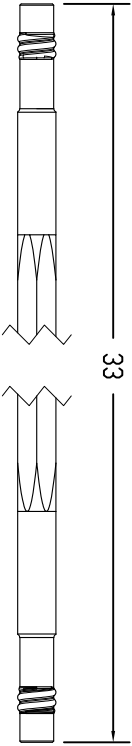
SG2 DRIVE STEEL EXTENSION QTY: 2
